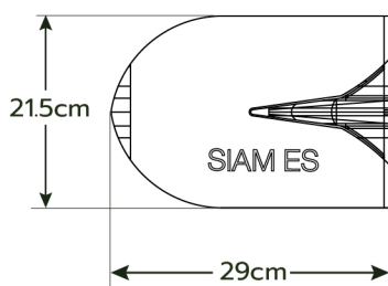
TOP VIEW Round Mouth Shovel
